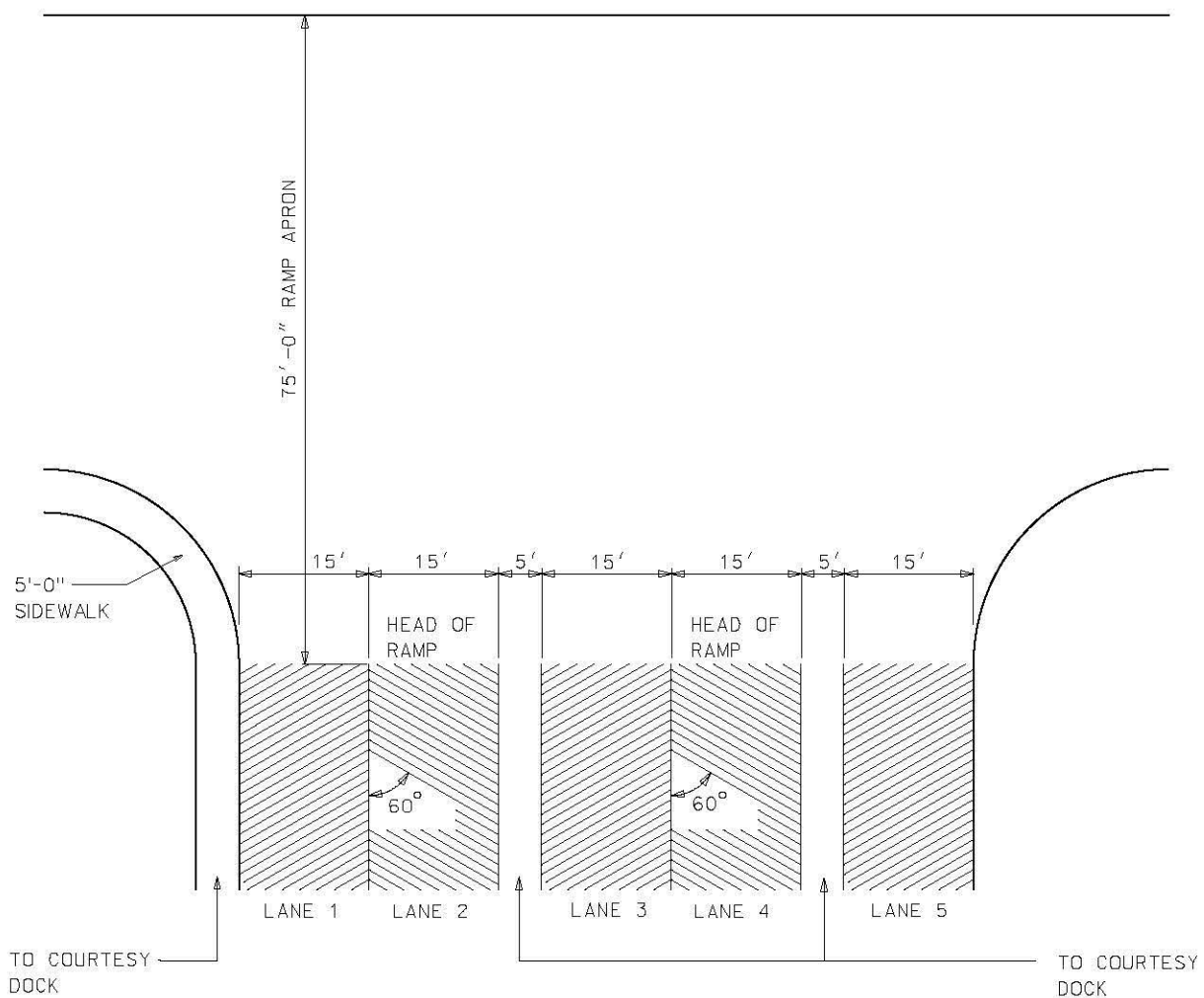
DRAWING NO. E-5 BOAT RAMP - MULTI-LANE
