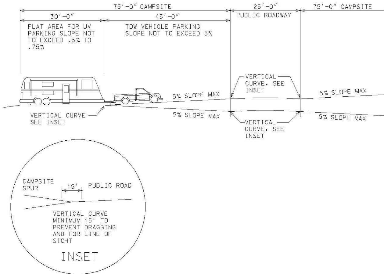
DRAWING NO. C-5 TYPICAL BACK-IN CAMPSITE SECTION
