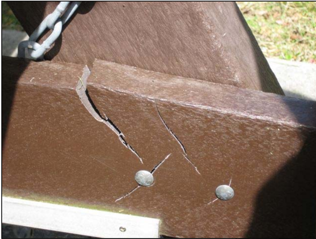
Cracking and splintering on seat supports
